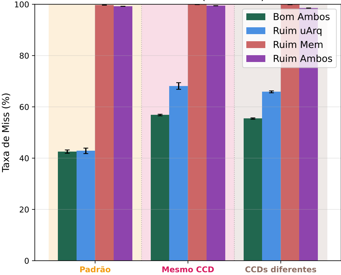
Taxa de Miss L1 (6 Threads)
