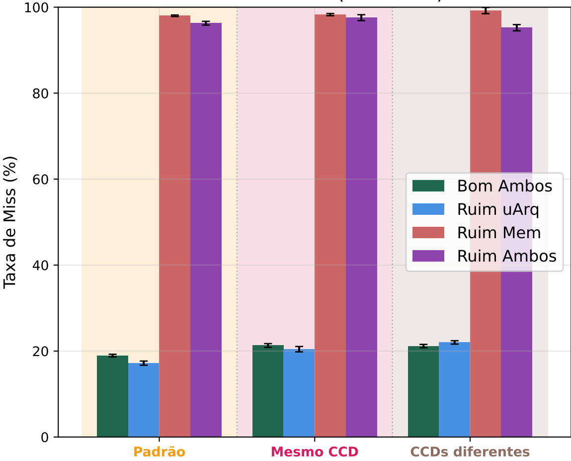
Taxa de Miss L2 (6 Threads)
