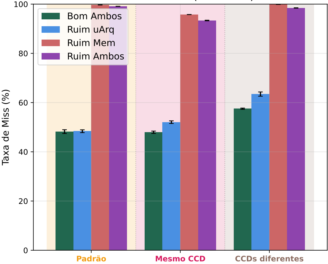
Taxa de Miss L1 (7 Threads)
