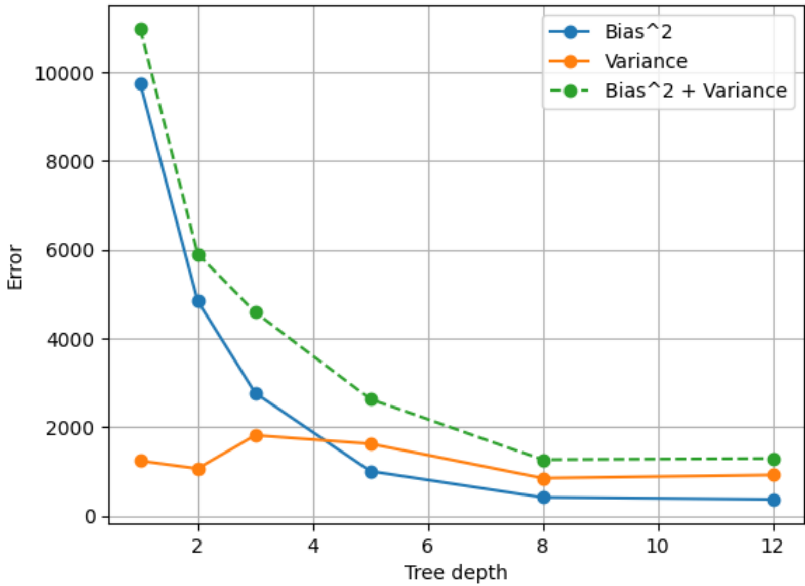
Bias-Variance Tradeoff in Decision Tree Regressor
