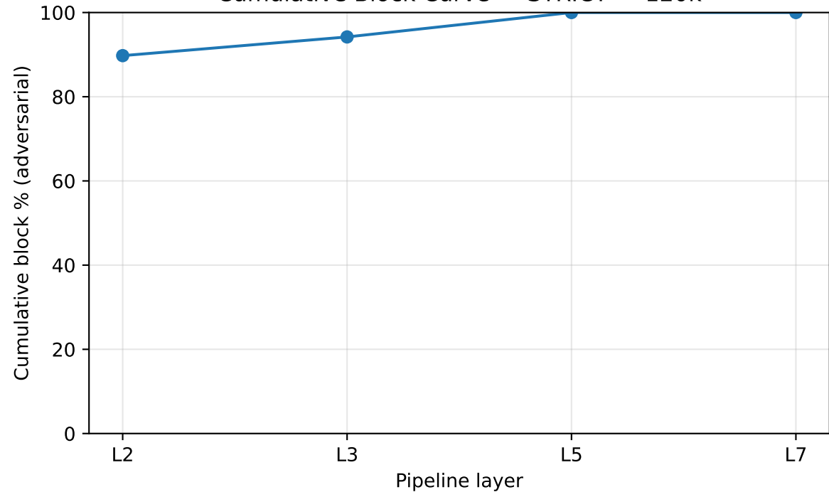
Cumulative Block Curve — STRICT — 120k
