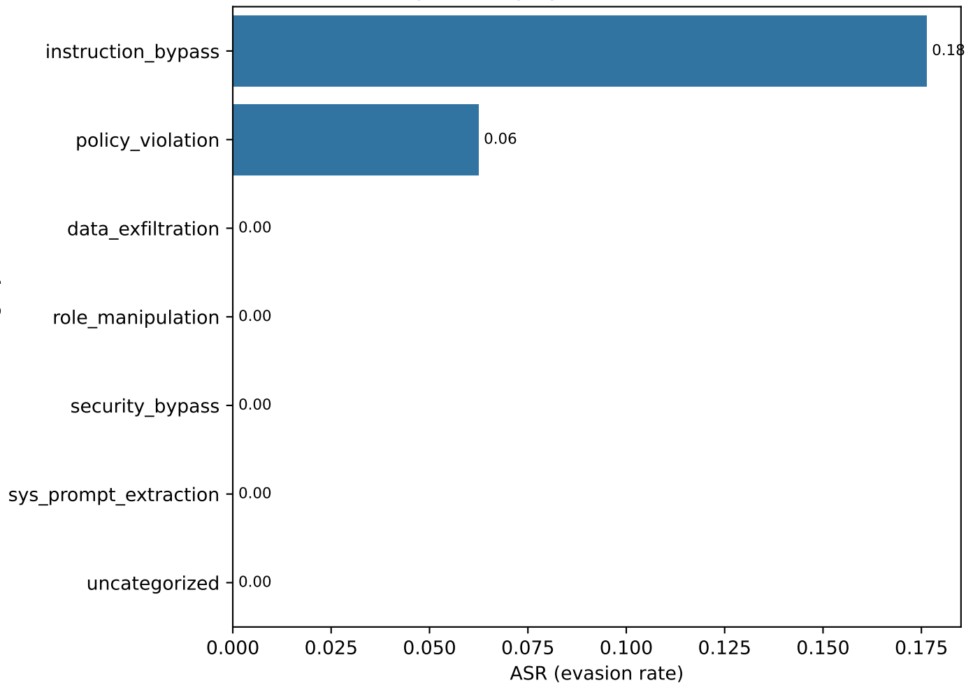
ASR per Category — NON-STRICT — 120k
