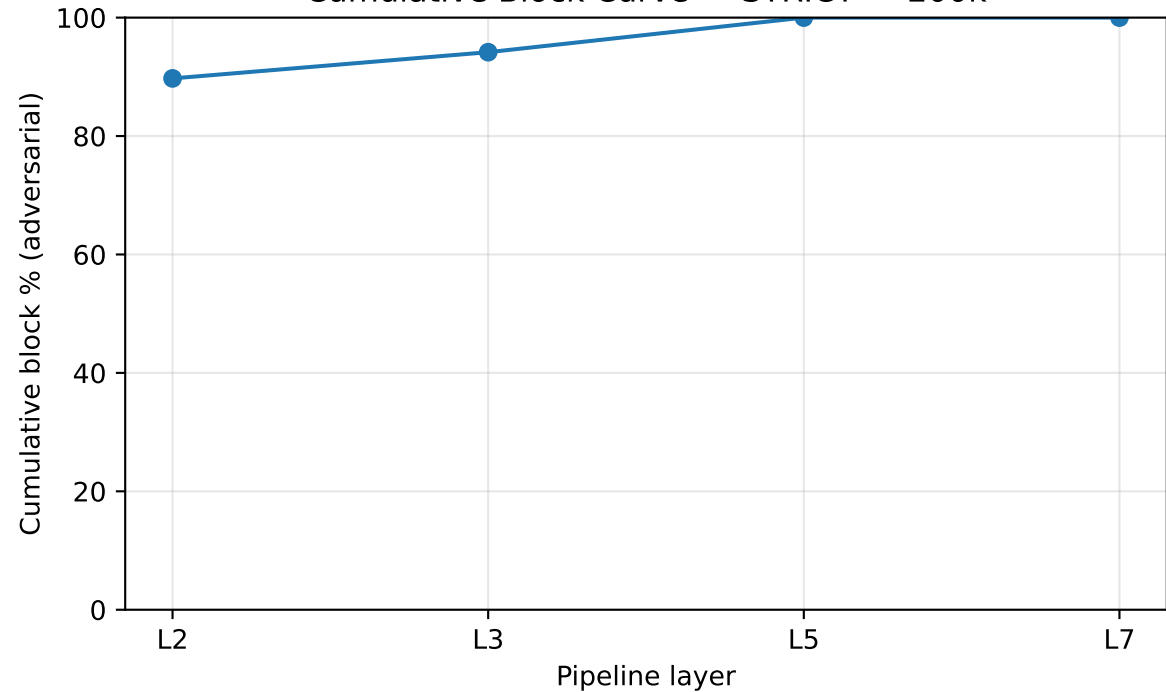
Cumulative Block Curve — STRICT — 200k
