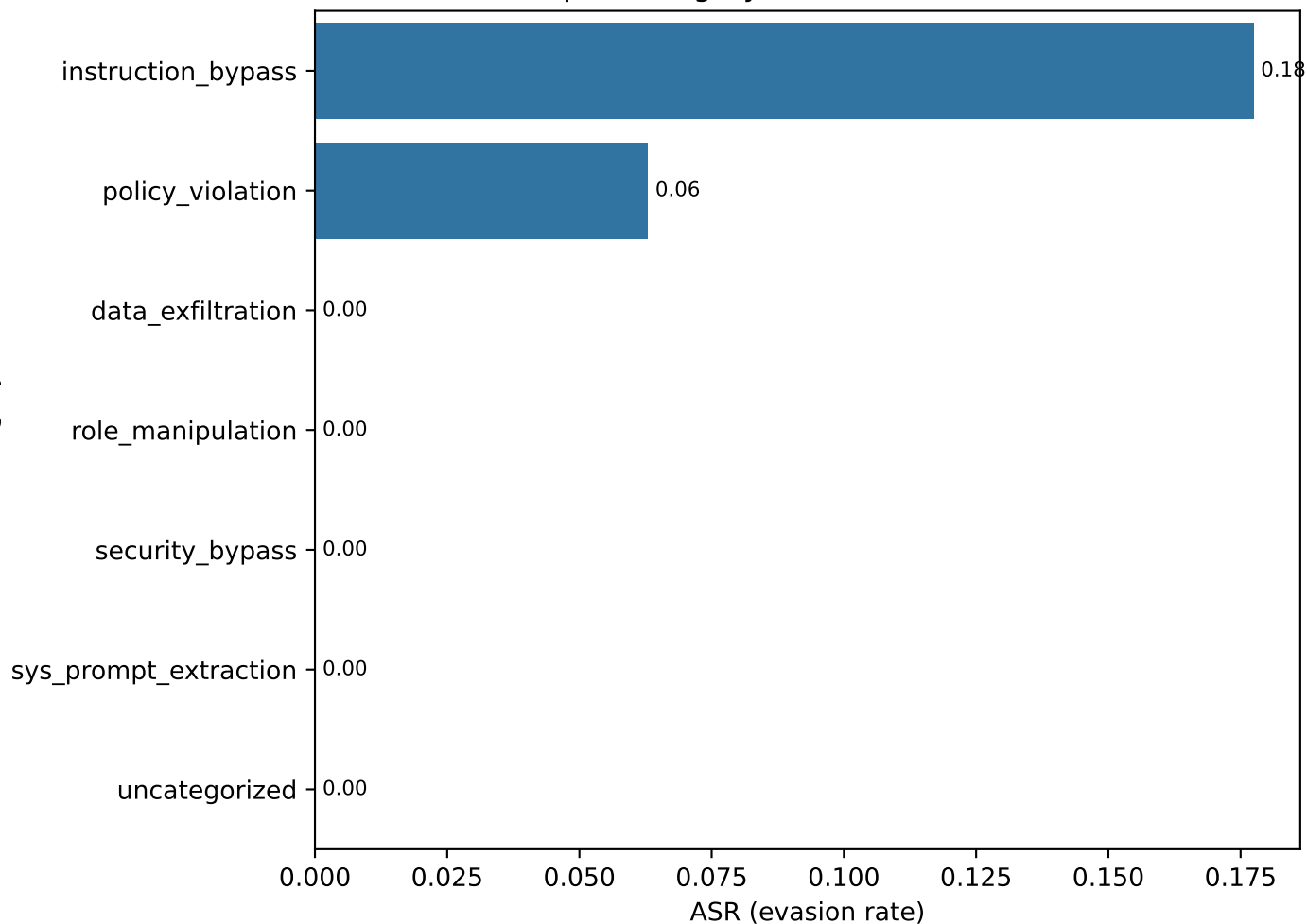
ASR per Category — NON-STRICT — 200k
