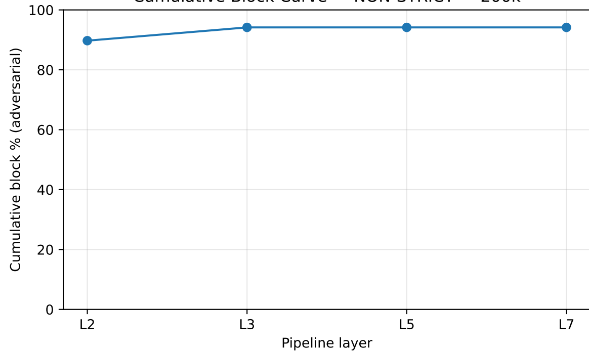
Cumulative Block Curve — NON-STRICT — 200k
