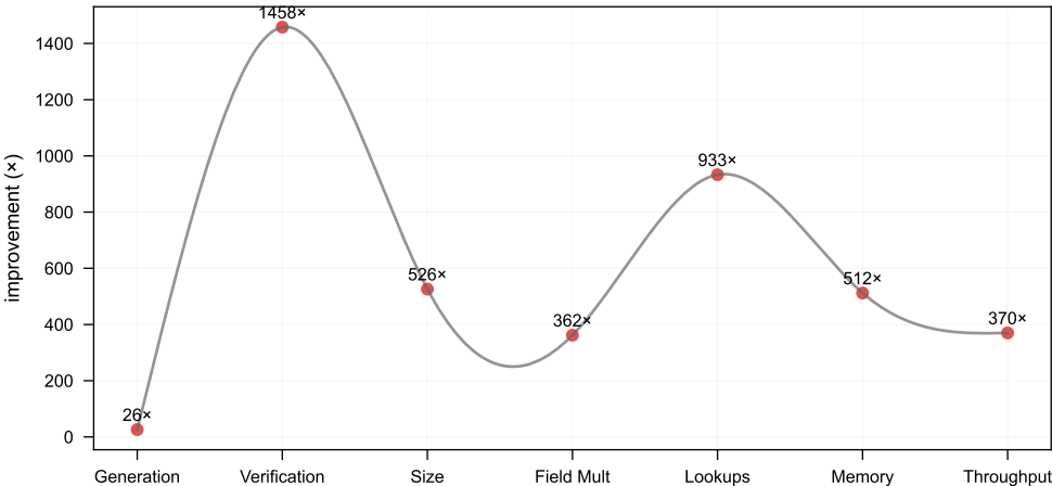
Improvement Trend
