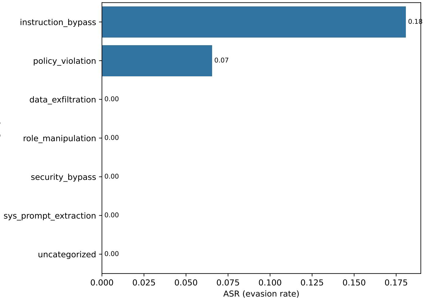
ASR per Category — NON-STRICT — 50k
