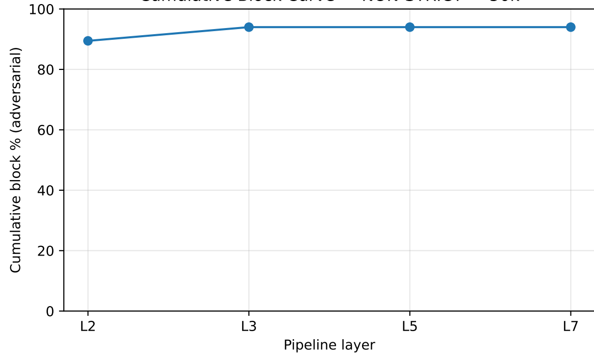
Cumulative Block Curve — NON-STRICT — 50k
