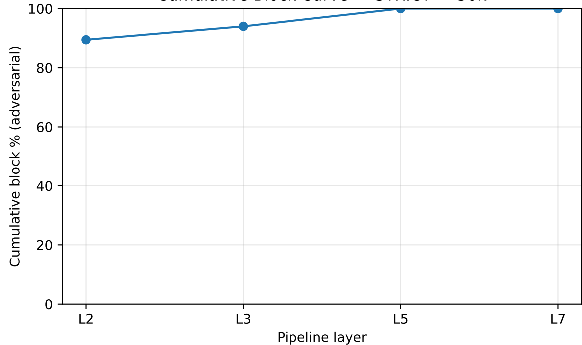
Cumulative Block Curve — STRICT — 50k
