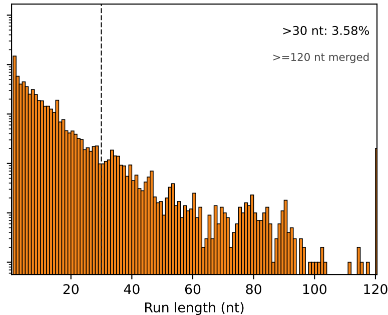
Exterior loop (E)
