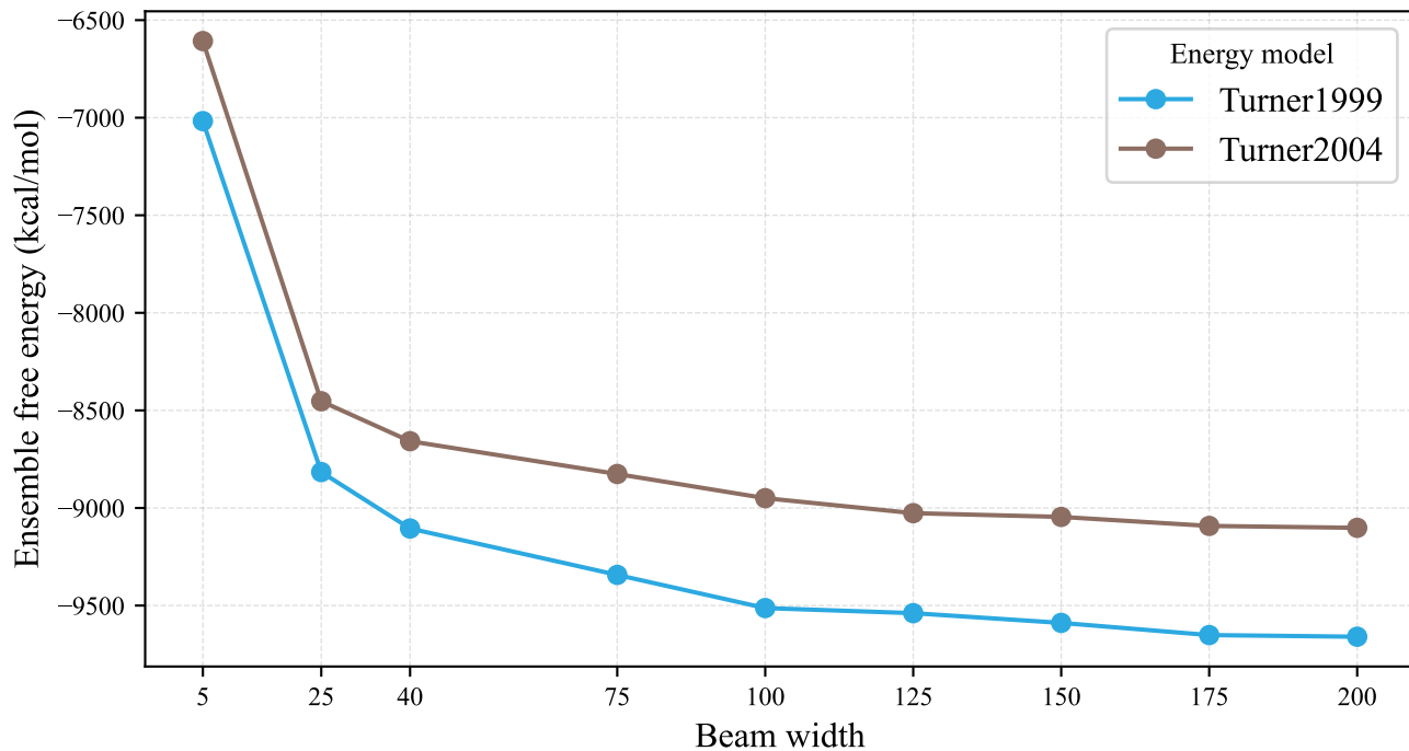
Effect of beam width on beam-pruned ensemble free energy for SARS-CoV-2.
