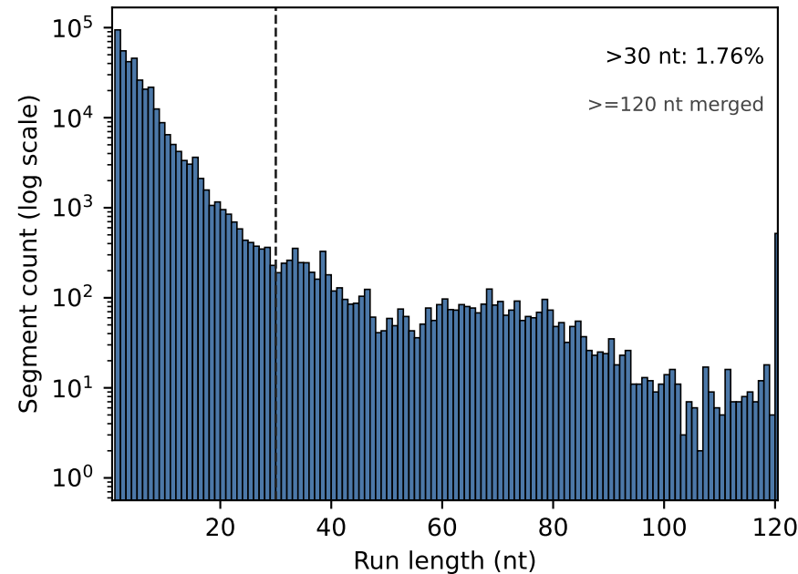
All unpaired contexts (HBIMEO)
