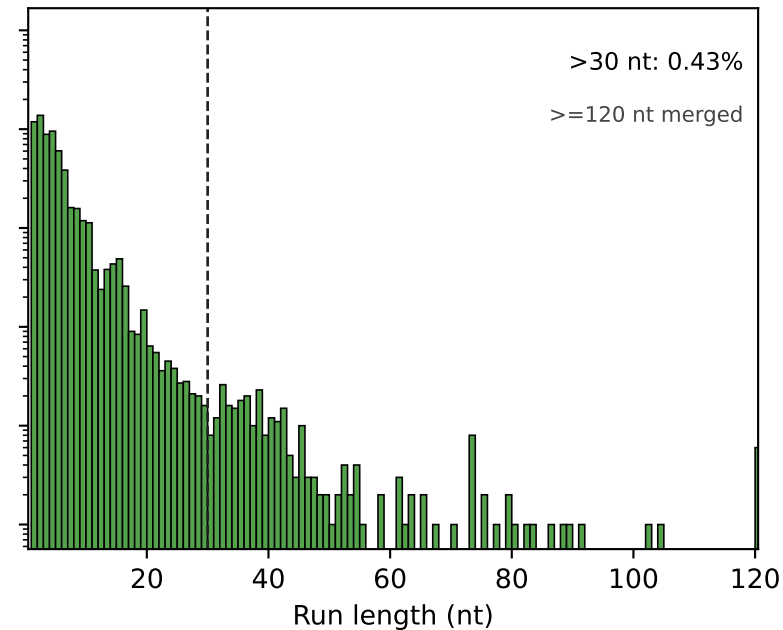
Multiloop unpaired (M)
