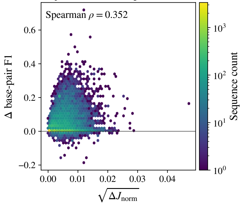
Objective and base-pair trade-off
