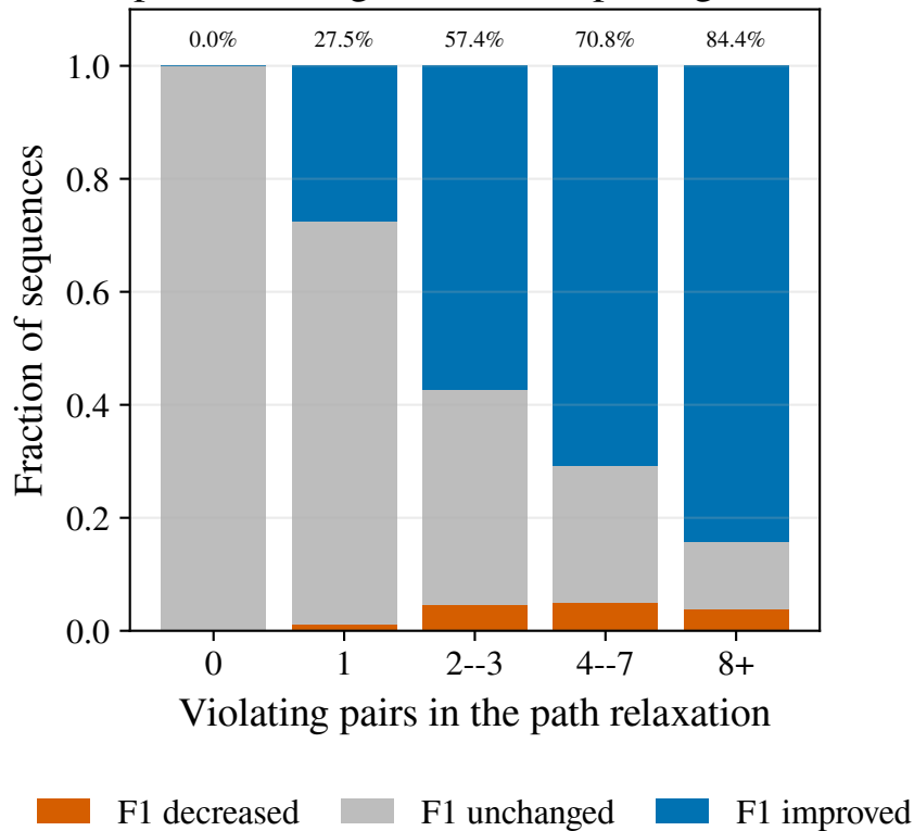
Base-pair F1 change after RNA pairing constraints
