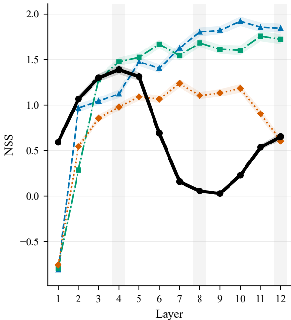
CLIP-B (CLIP ViT-B/16) DINO-B (DINO ViT-B/16) DINO-S (DINO ViT-S/16) DeiT/SL (DeiT/SL ViT-S/16)
