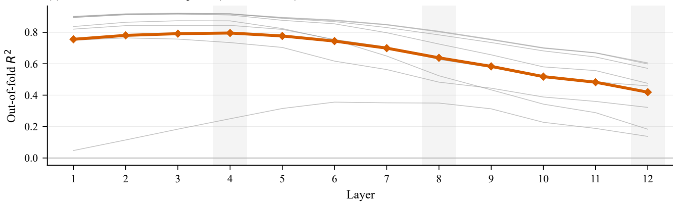
(c) Low-level visual-feature probe (8-feature mean)
