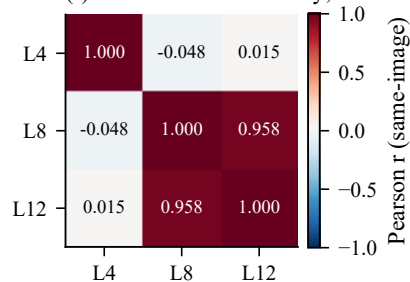
(f) L8-L12 attend similarly; L4 differs
