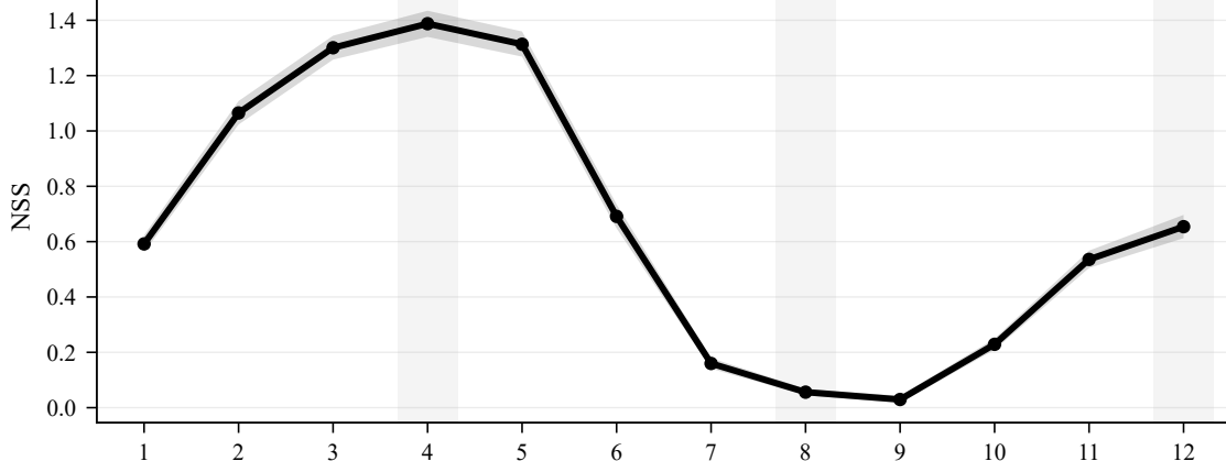
(b) Semantic-attribute probe (all 12 attributes)
