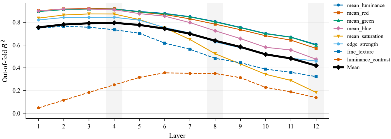
(c) Low-level visual-feature probe (all 8 features)
