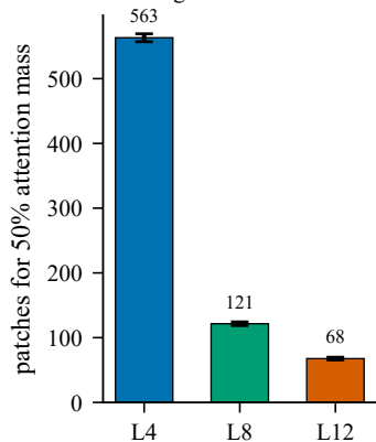
(f) Number of patches covering 50% attention mass
