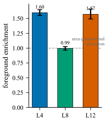
(g) Foreground enrichment relative to area
