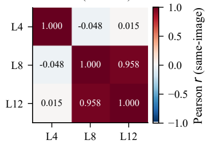
(h) Same-image spatial correlation (Pearson r )
