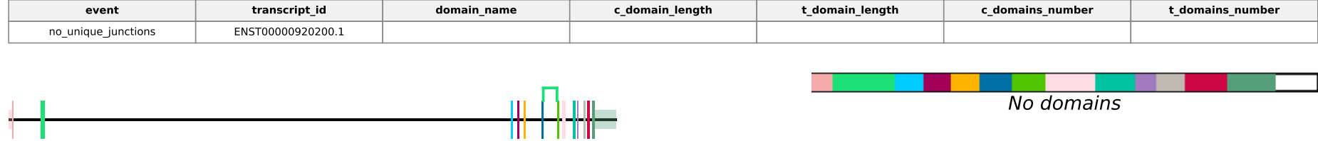
Transcript: ENST00000920202.1 | Protein: ENSP00000590261.1
