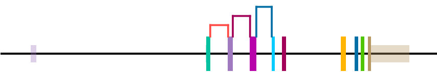
Transcript: ENST00000880296.1 | Protein: ENSP00000550355.1
