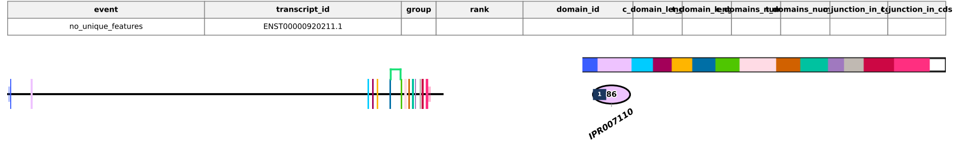
Transcript: ENST00000920211.1 | Protein: ENSP00000590270.1
