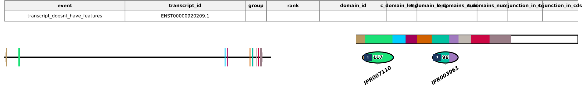
Transcript: ENST00000920209.1 | Protein: ENSP00000590268.1
