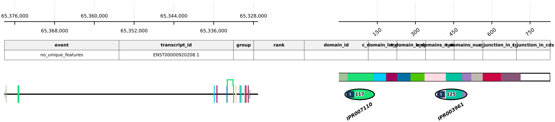
Transcript: ENST00000920208.1 | Protein: ENSP00000590267.1
