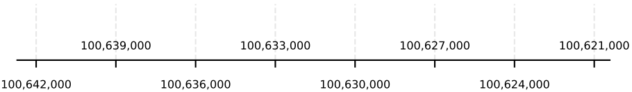
Genomic Position (bp)
