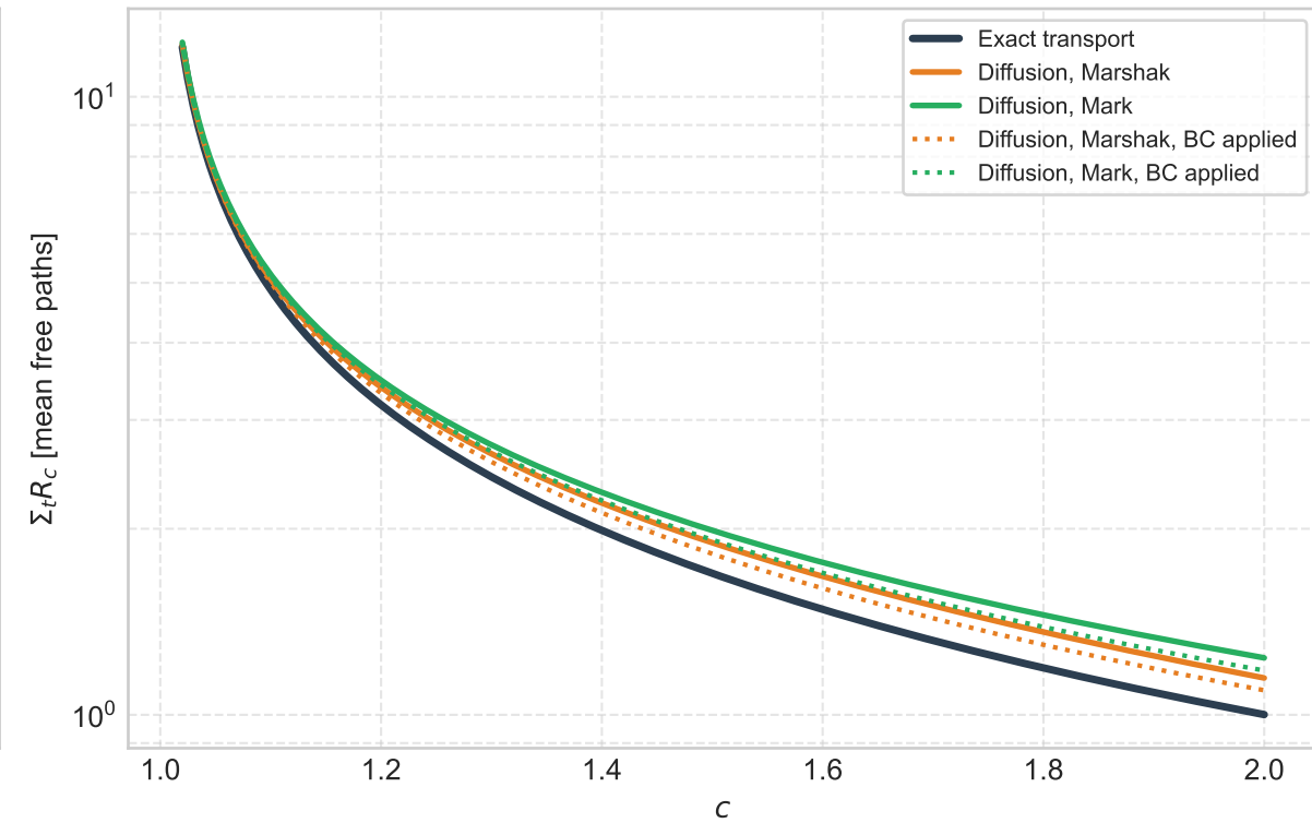
Departure from Exact Transport, \Sigma_t R_c
