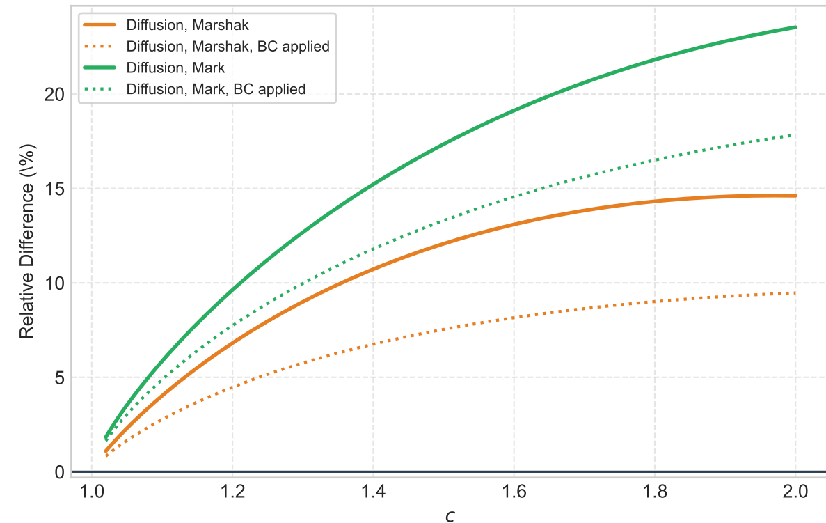
Departure from Exact Transport, \Sigma_t R_c
