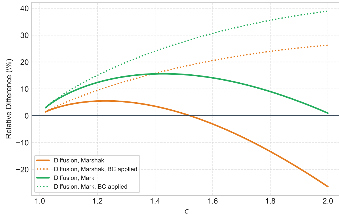
Departure from Exact Transport, a/2
