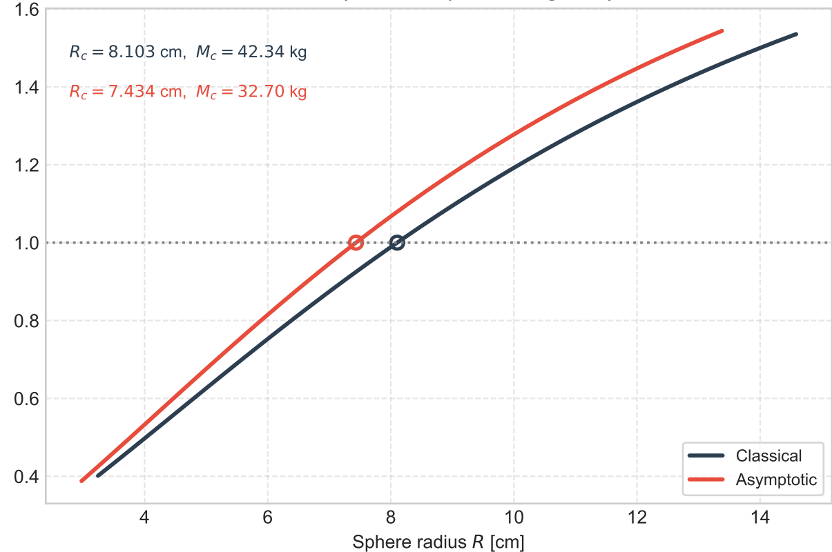
U-235 ( c = 1.30 , \rho = 19.0 \text{ g/cm}^3 )
