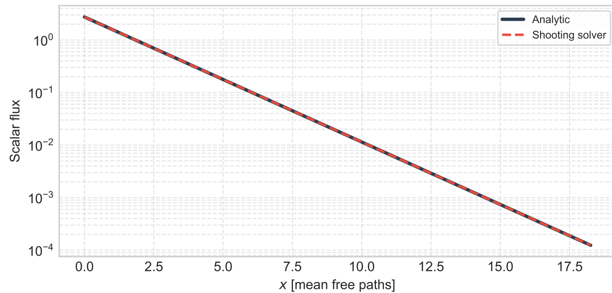
Classical diffusion, c = 0.9
