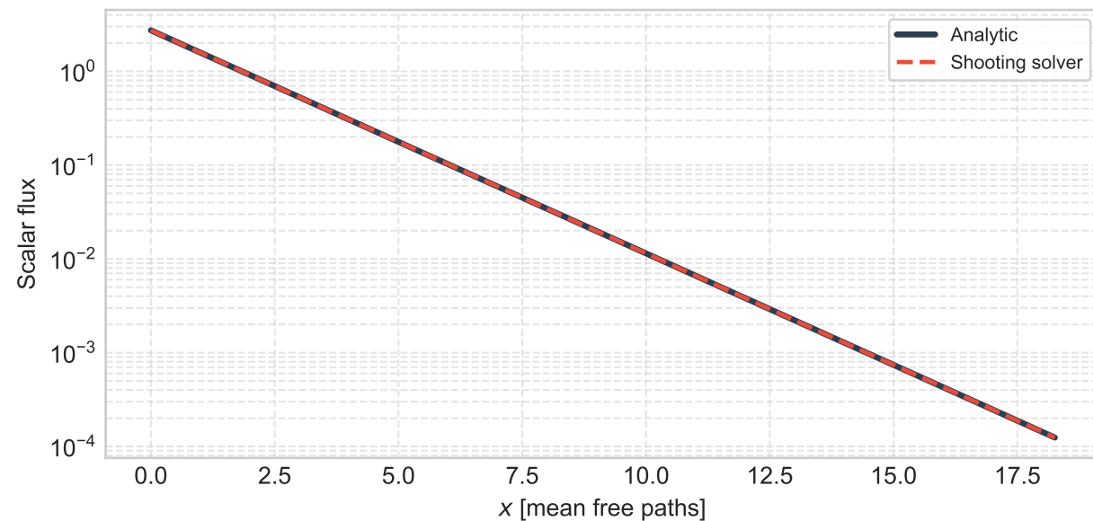
Classical diffusion, c = 0.9
