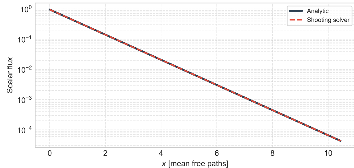
Asymptotic diffusion, c = 0.7
