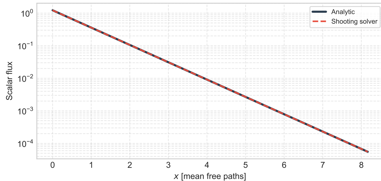
Classical diffusion, c = 0.7
