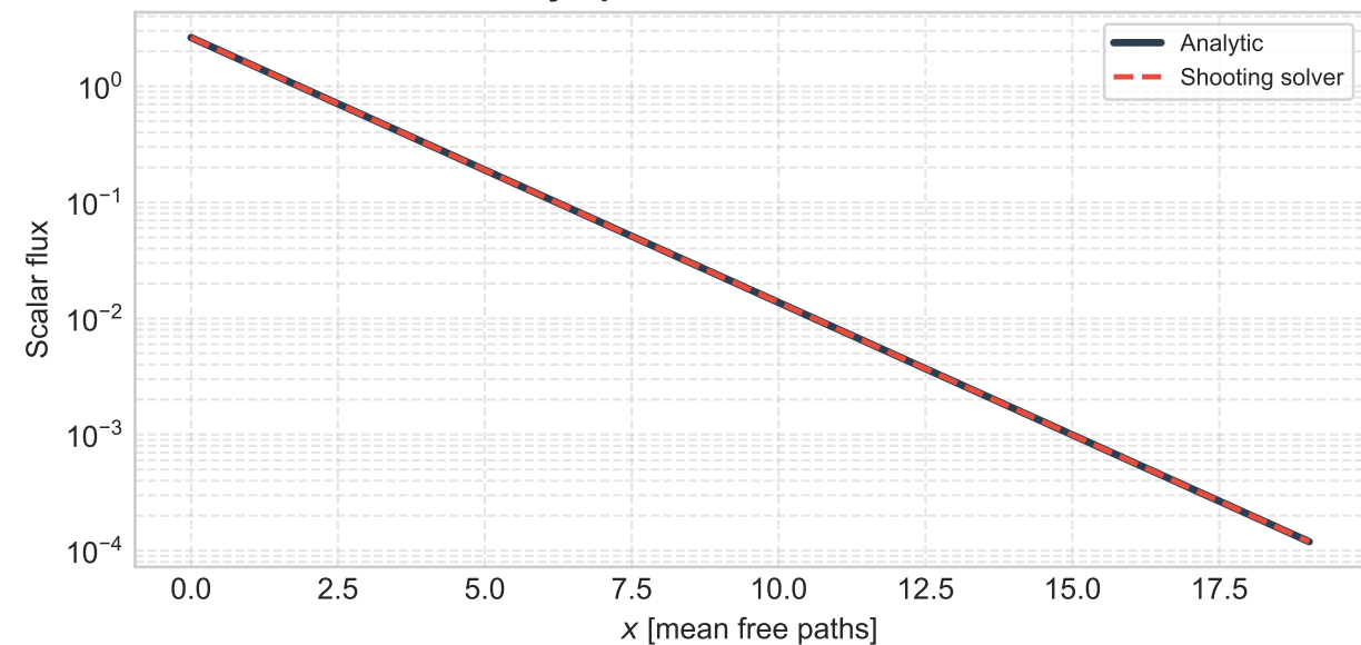
Asymptotic diffusion, c = 0.9
