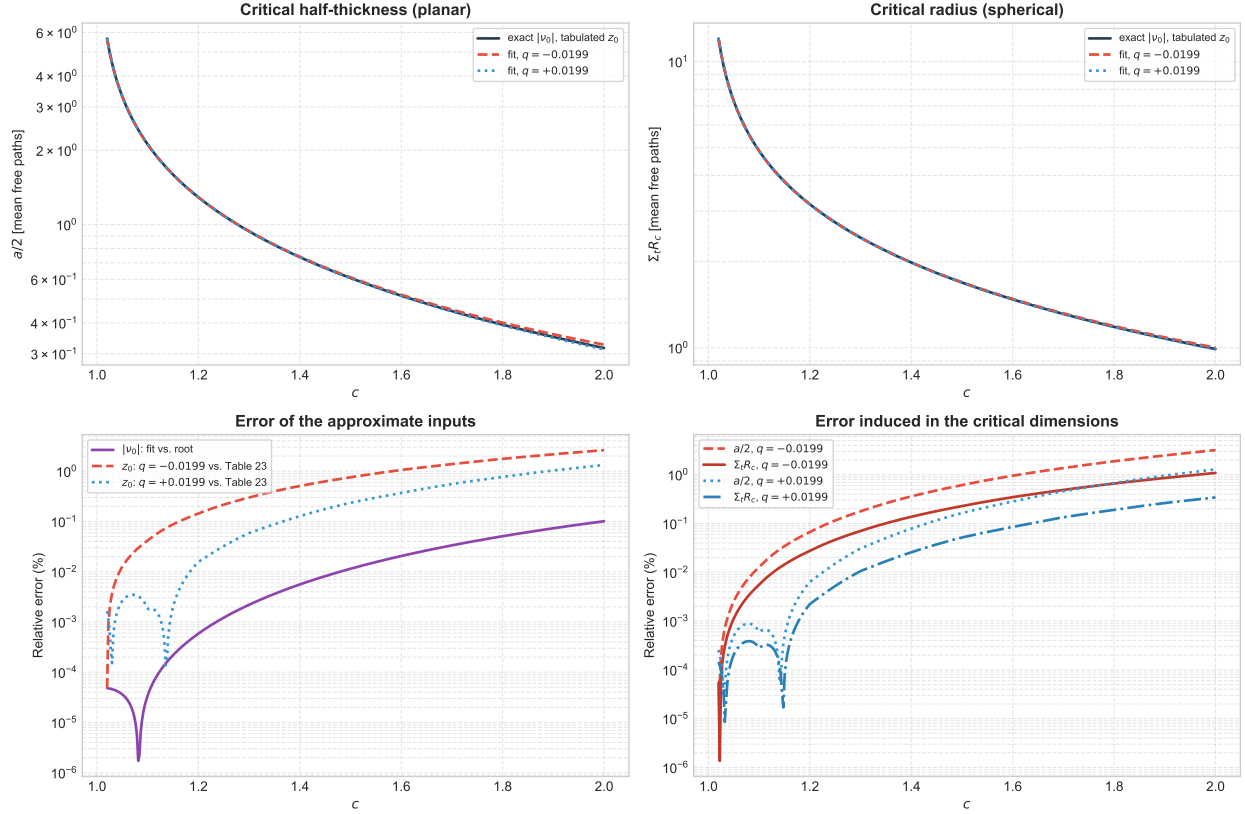
Figure 6: Critical half-thickness and radius for 1.02 < c < 2 (top), and the errors of the approximate inputs and of the resulting dimensions (bottom).
