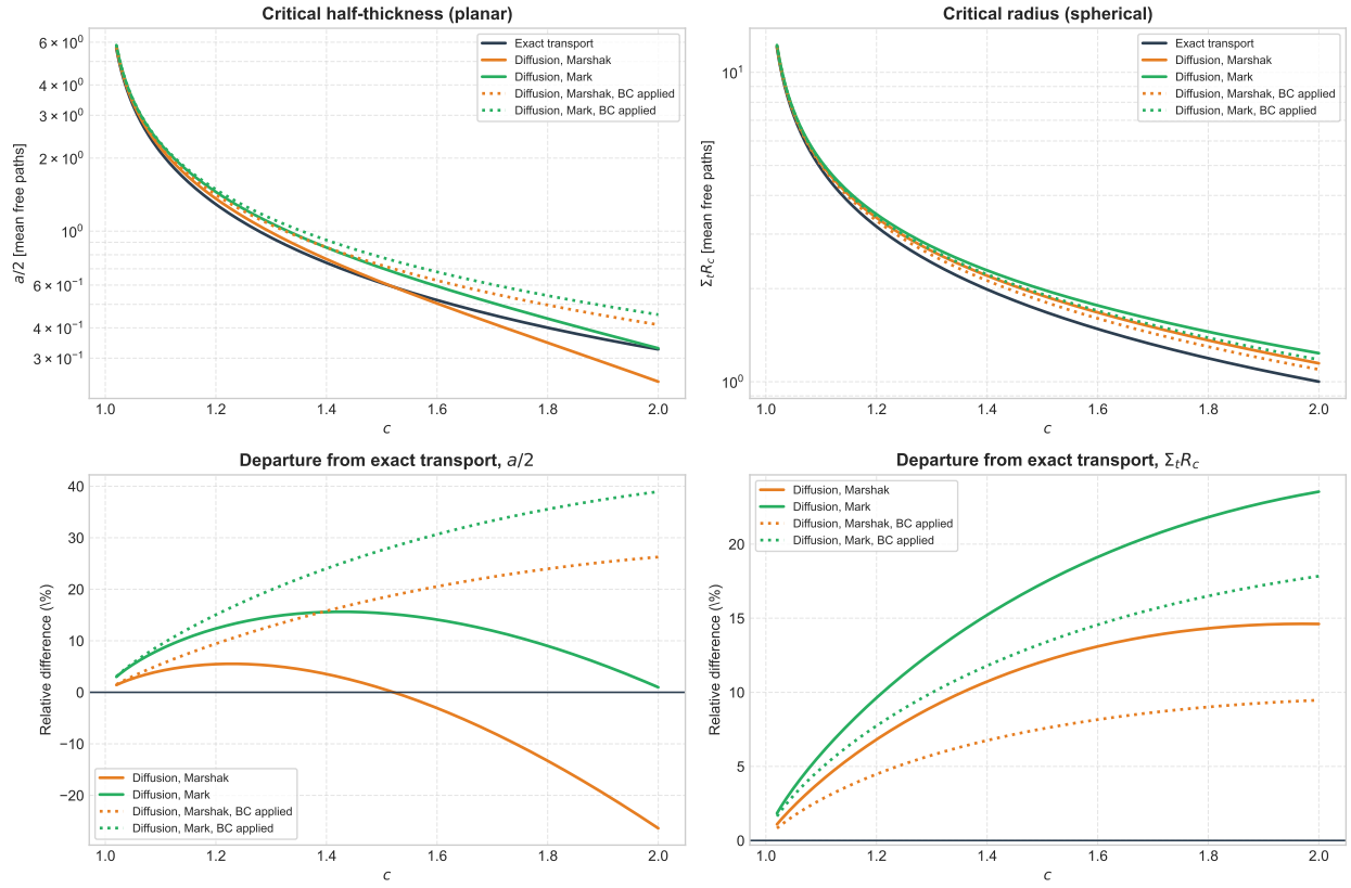
Figure 7: Exact transport against Marshak and Mark diffusion (top), and the signed departure of each from transport (bottom). Dotted curves impose the boundary condition on the flux shape instead of using an extrapolated zero.
