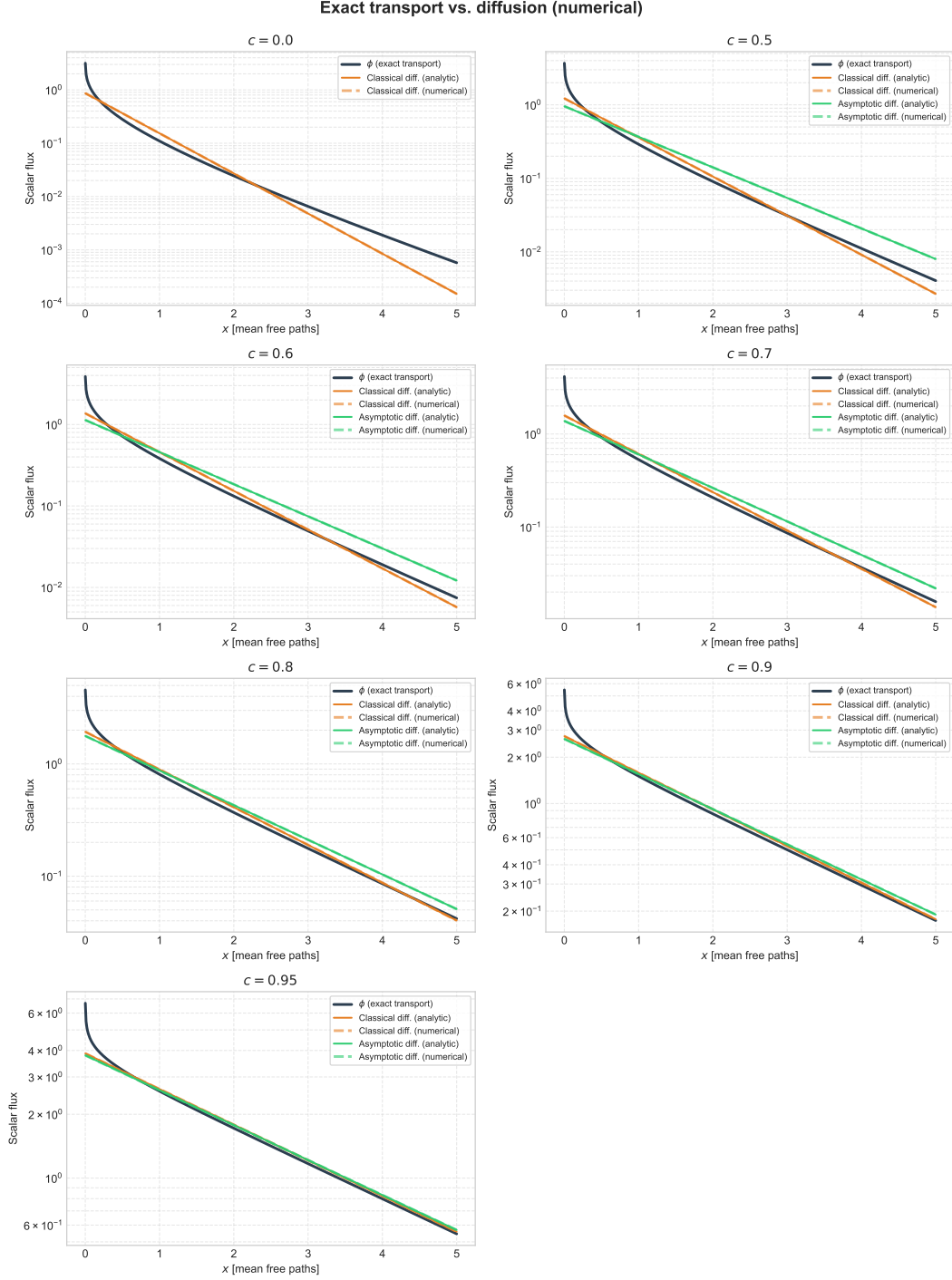
Figure 1: Exact scalar flux against the classical and asymptotic diffusion approximations, for c = 0, 0.5, 0.6, 0.7, 0.8, 0.9, 0.95 . Each approximation appears both as its closed form and as the numerical solution of Question 2; the two agree to 2 \times 10^{-8} \% and are indistinguishable here.
