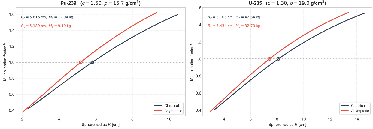
Figure 11: Multiplication factor against sphere radius for the two fissile materials, both approximations. The circles mark the k = 1 crossing.
