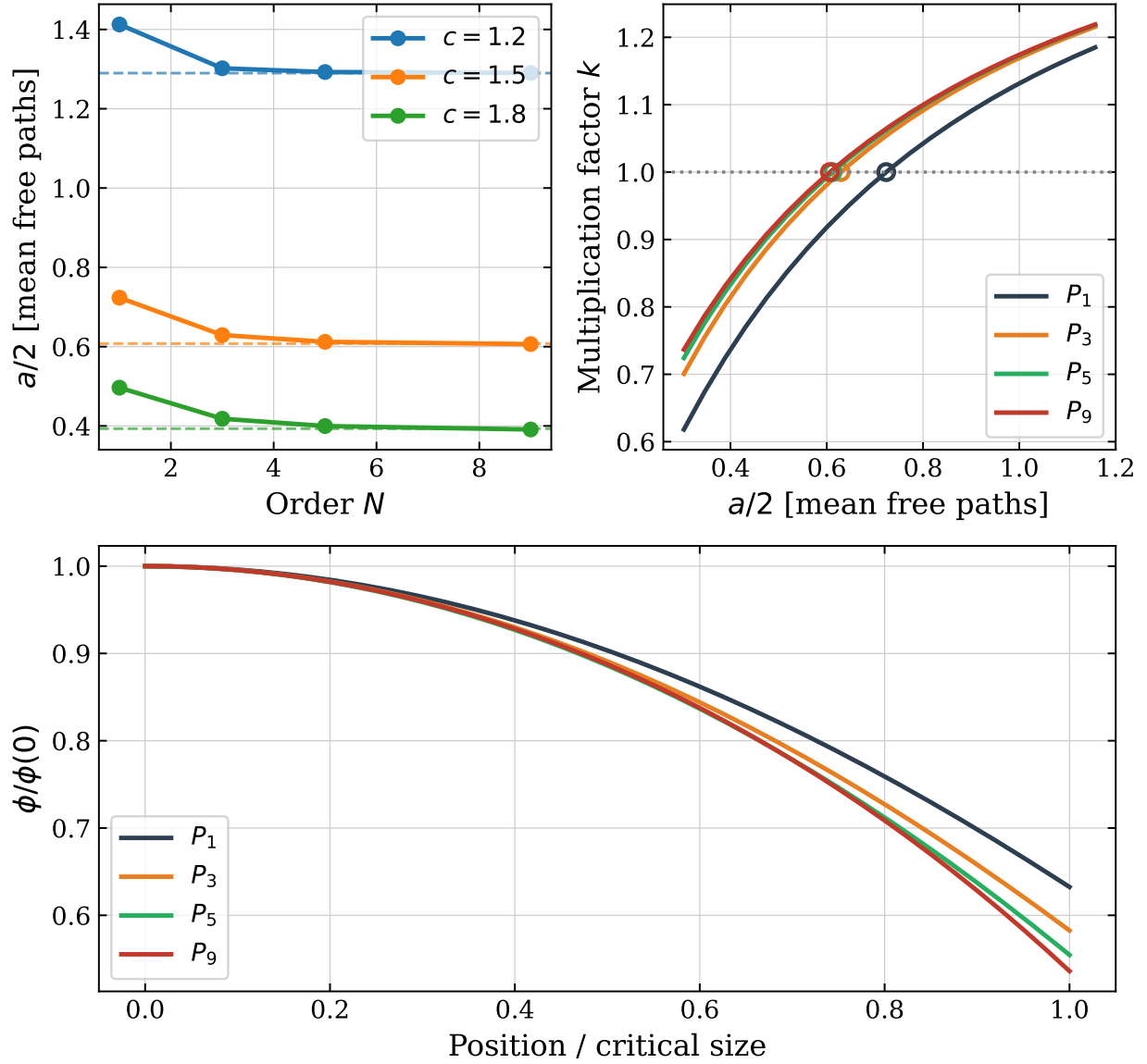
Figure 3: Top left: convergence of (a/2)_{\text{crit}} with N , dashed lines the exact-transport values. Top right: k against half-thickness at c = 1.5 , circles the k = 1 crossings, which for P_3 , P_5 and P_9 are already almost on top of one another. Beneath them: the normalised critical flux - as in Question 3, the order changes the surface value and not the interior shape.
