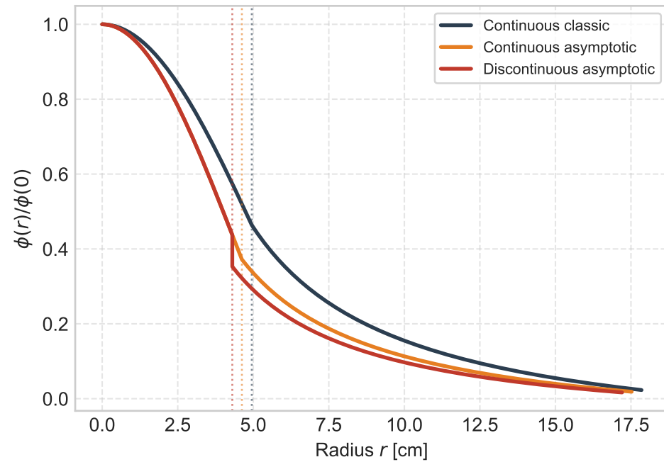
Pu-239 + Iron, d = 3 mfp
