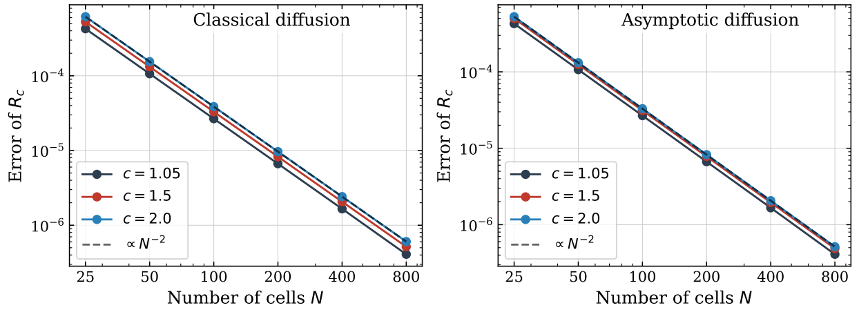
Figure 10: Mesh convergence of the critical radius, following the second-order guide \propto N^{-2} at every refinement.
