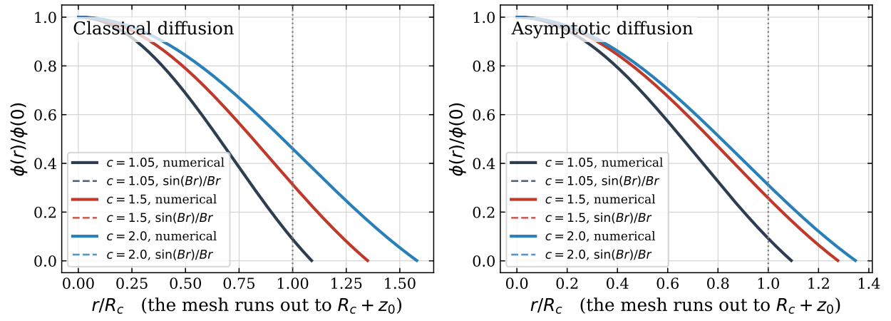
Figure 11: Converged critical flux (solid) against the fundamental mode \sin(Br)/Br (dashed), normalised at the centre. The mesh continues past r/R_c = 1 to the extrapolated radius, where the flux is driven to zero.
