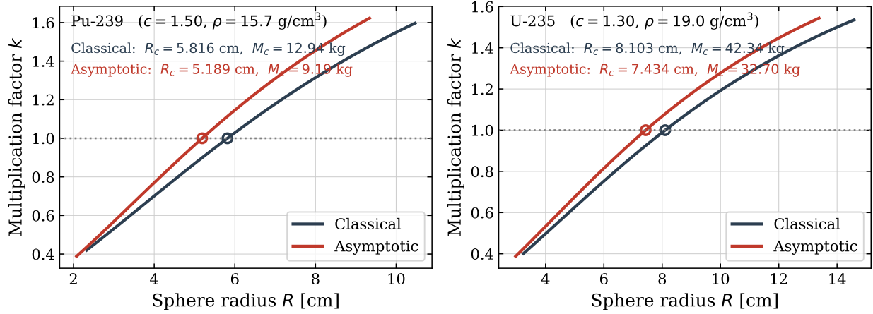
Figure 12: Multiplication factor against sphere radius for the two fissile materials, both approximations. The circles mark the k = 1 crossing. Sorry for the captions over the graphs, it's unprofessional but I didn't get to erasing them.
