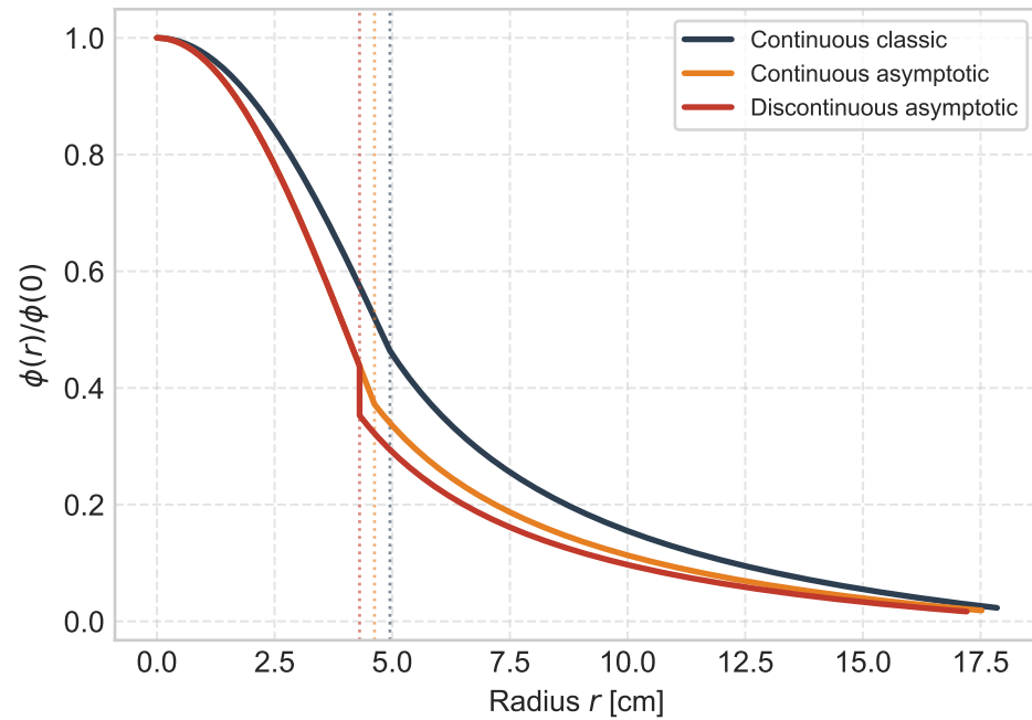
Pu-239 + Iron, d = 3 mfp
