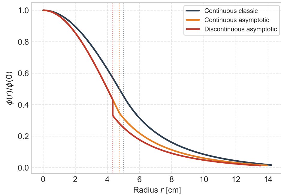
Pu-239 + Water, d = 3 mfp
