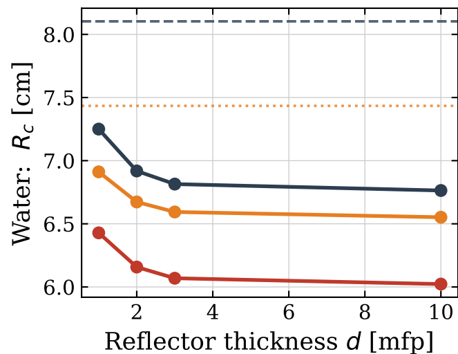
U-235
