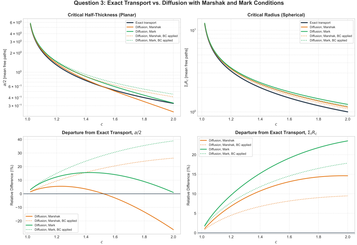
Figure 8: Exact transport against diffusion with Marshak and Mark boundary conditions (top), and the signed departure of each diffusion result from the transport one (bottom). Dotted curves impose the boundary condition on the flux shape instead of using an extrapolated zero.
