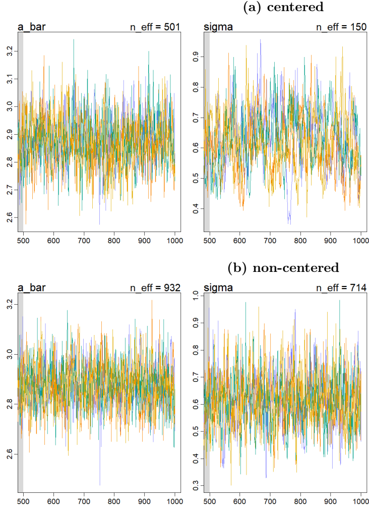
Figure 1: Trace plots for \bar{\alpha} and \sigma , warmup excluded. Both are stationary — neither is broken — but they are not equally good. The centered \sigma trace makes slow excursions that last tens of iterations, drifting low around iteration 800 and high around 900. The non-centered trace oscillates rapidly with no such drift. Slow excursions mean successive draws carry nearly the same information, which is exactly what a low effective sample size reports.
