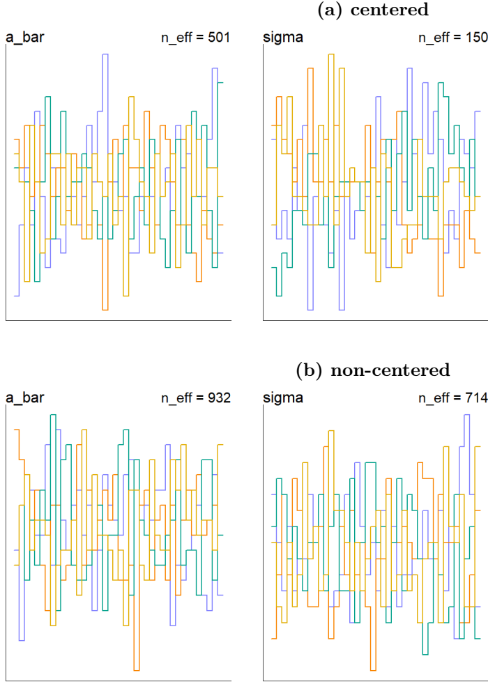
Figure 2: Trace rank plots. Look at the \sigma panel of (a): one chain holds far more than its share of the lowest ranks at the left edge, and another spikes at the highest ranks on the right. Those are chains that spent too long in one region — the same slow excursions the trace plot showed, now visible as an imbalance rather than as a wiggle. In (b) the four histograms interleave much more evenly.
