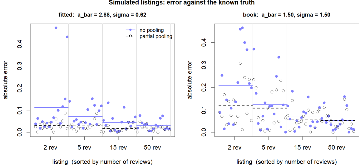
Figure 6: Absolute error for each simulated listing against ground truth p_i^{\text{true}} . Blue points and solid lines represent no pooling; open circles and dashed black lines represent partial pooling. Left: Fitted Airbnb scenario ( \bar{\alpha} = 2.88, \sigma = 0.62 ). Right: Textbook scenario ( \bar{\alpha} = 1.50, \sigma = 1.50 ). Partial pooling prevents large errors in low-review listings while matching no-pooling performance when evidence ( N_i = 50 ) is high.
