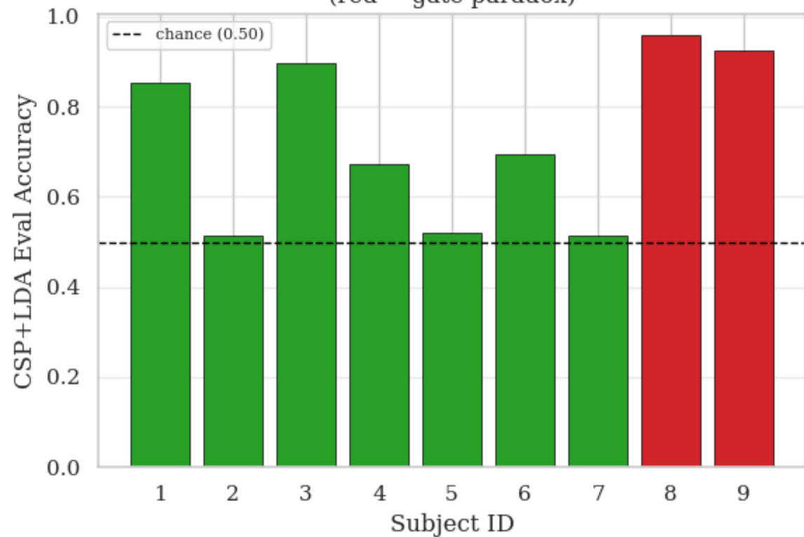
Per-Subject Eval Accuracy (red = gate paradox)
