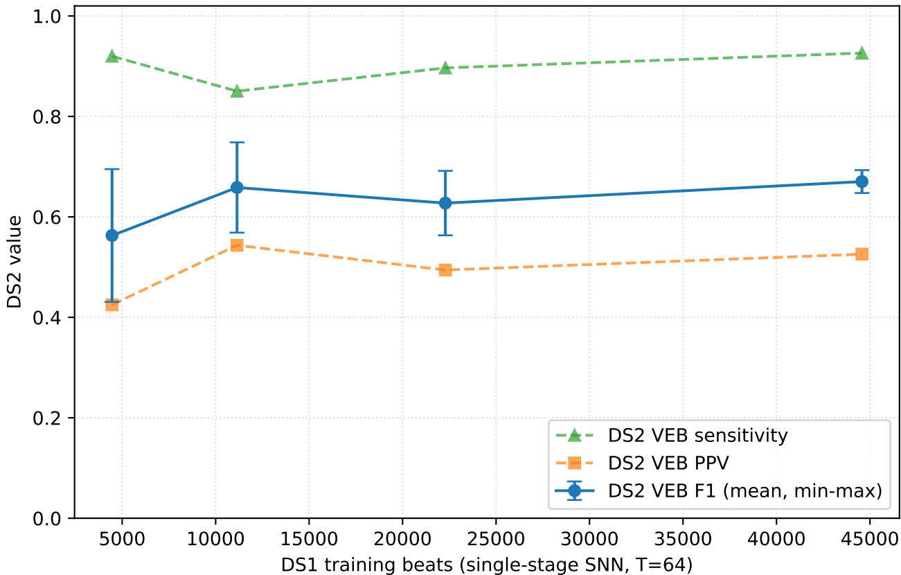
Learning curve: DS2 VEB detection vs training-set size
