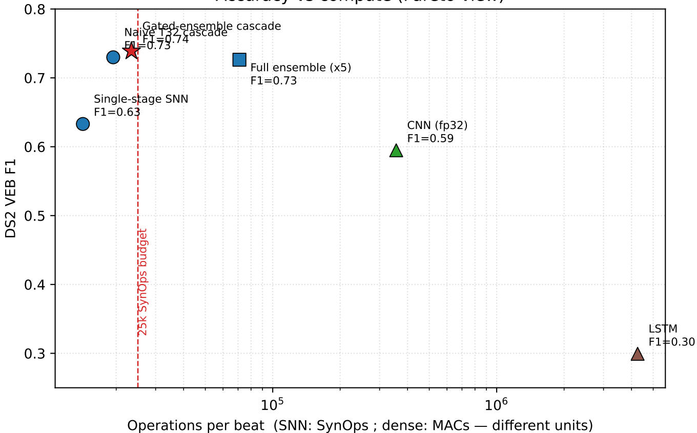
Accuracy vs compute (Pareto view)
