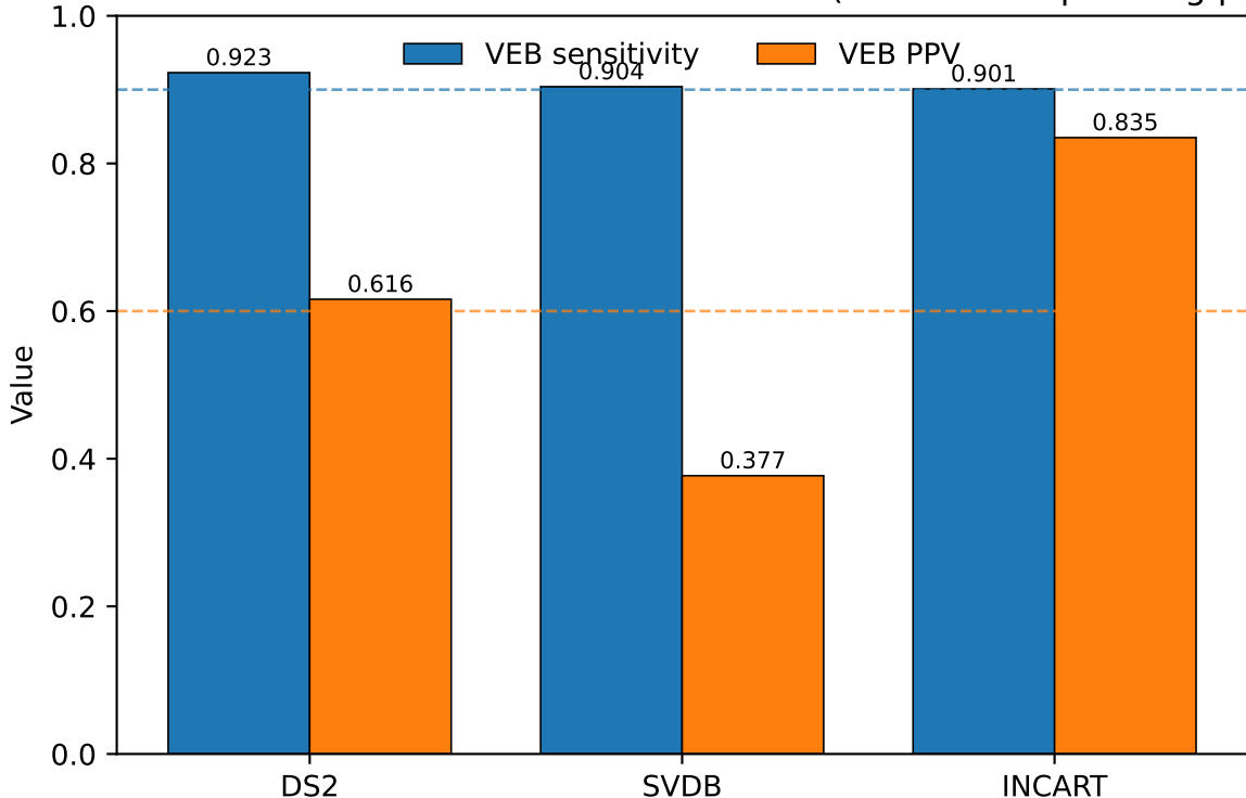
Gated cascade: cross-database VEB transfer (one frozen operating point)
