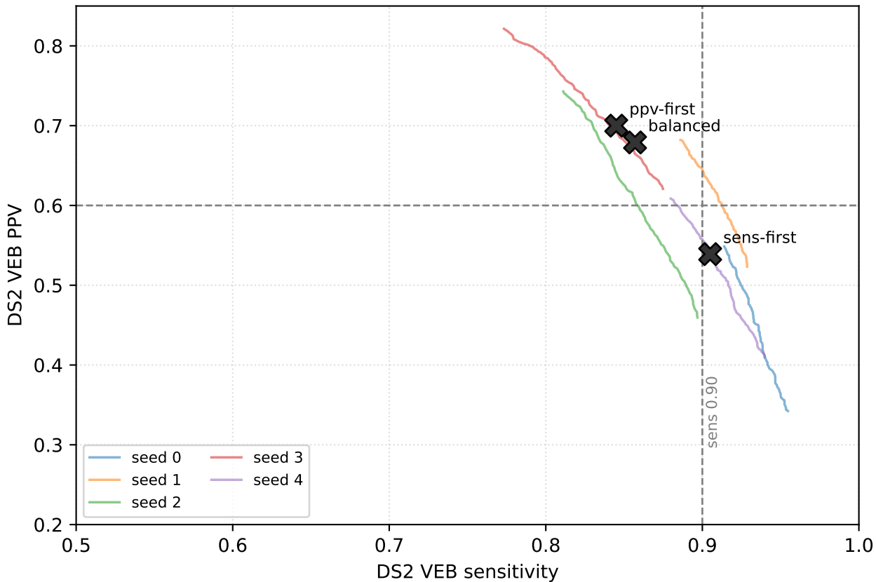
Single-stage sensitivity-PPV frontier (per seed, DS2 sweep)
