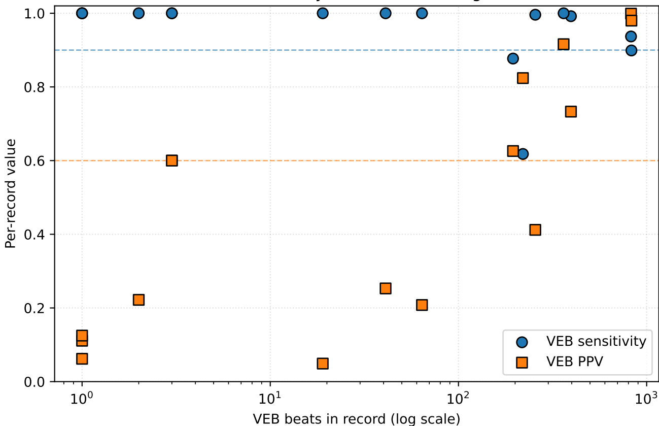
Per-record VEB sensitivity and PPV on DS2 (gated cascade)
