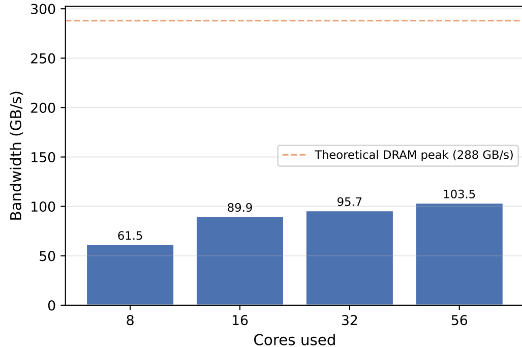
DRAM bandwidth vs core count
