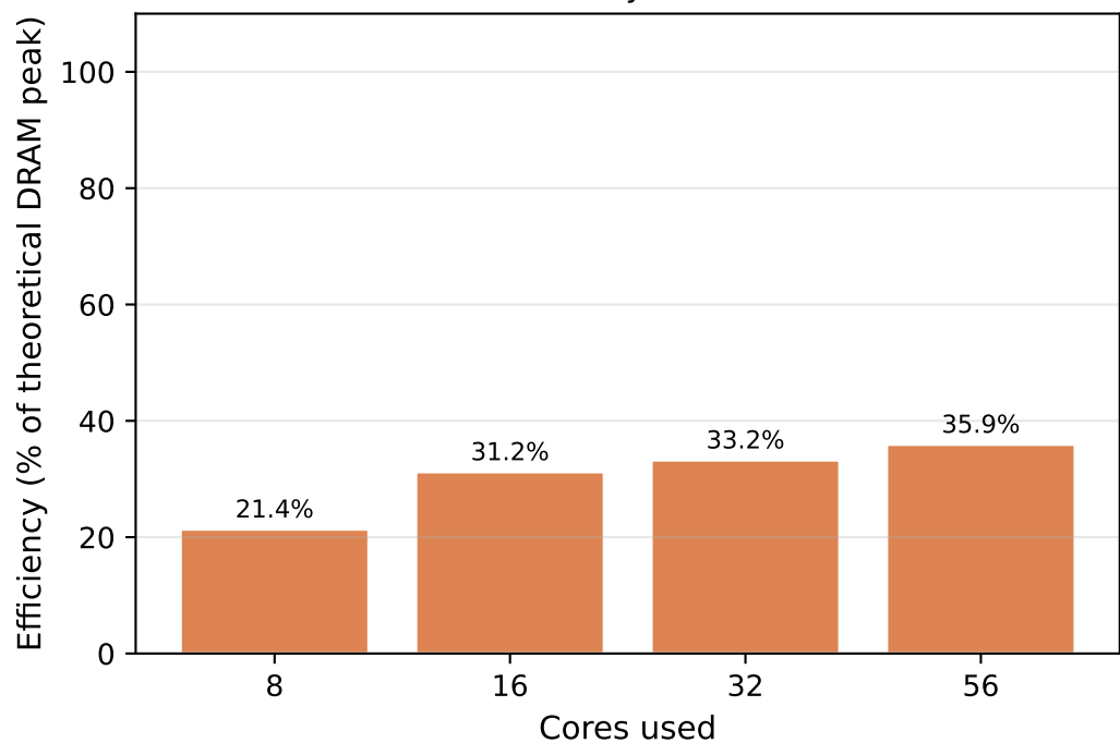
DRAM efficiency vs core count
