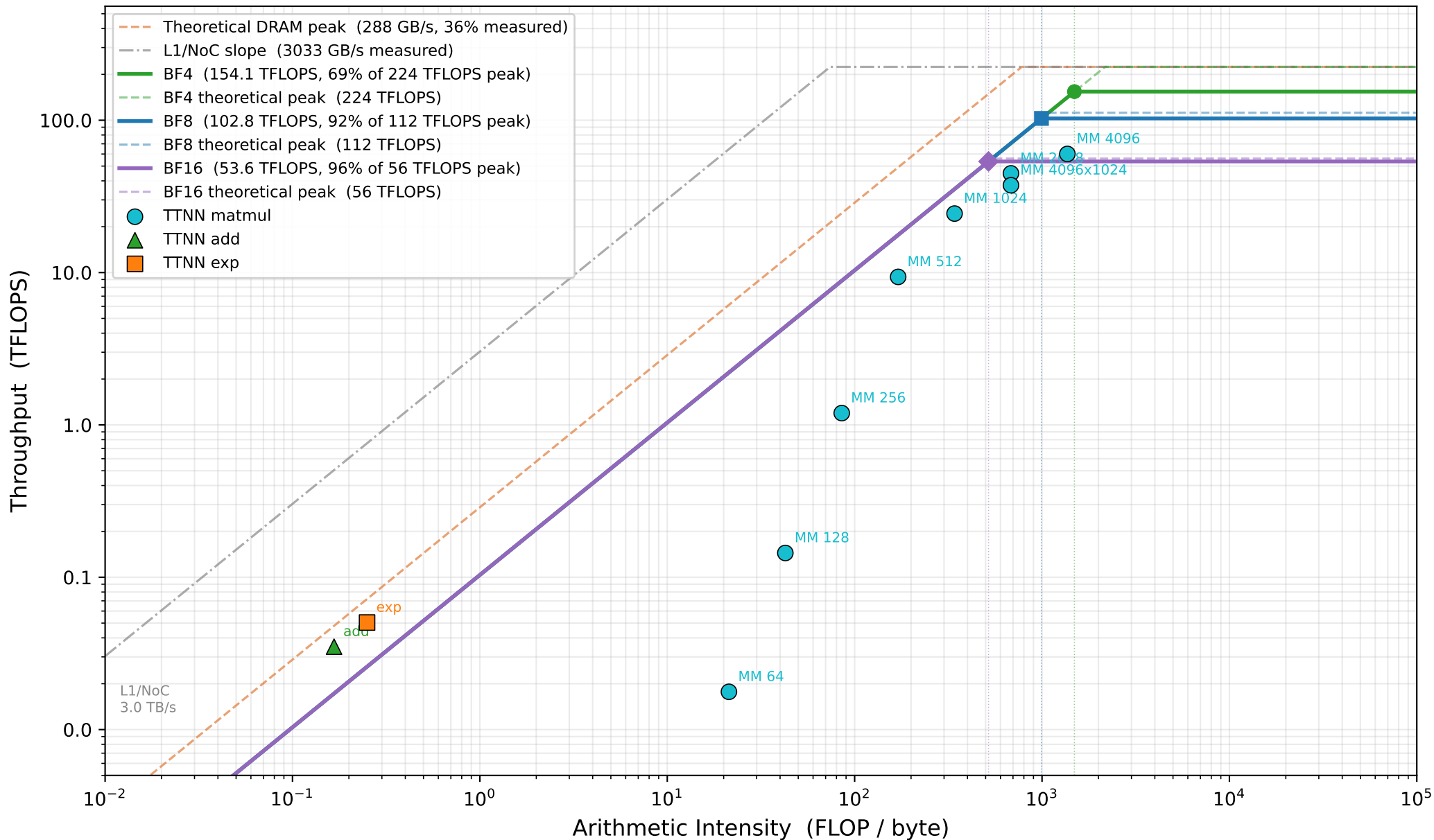
Empirical Roofline Model — Wormhole n300, single chip (BF4/BF8/BF16 format sweep, each at its standard fidelity; dashed = theoretical peak)
