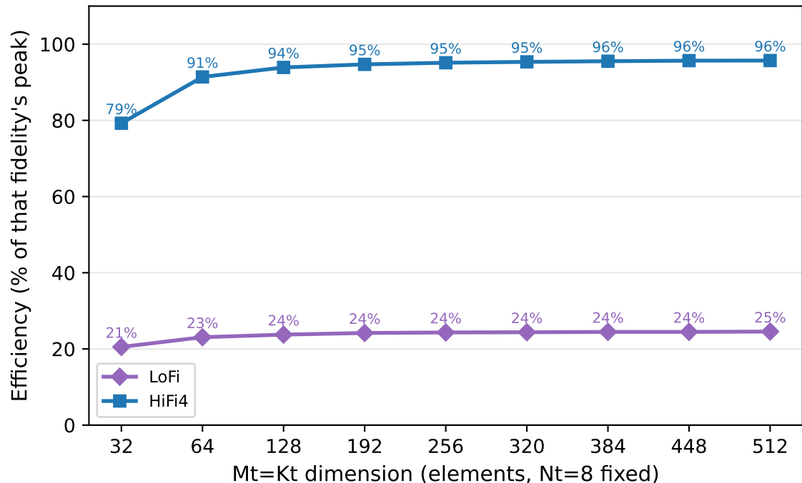
BF16: efficiency vs matrix size
