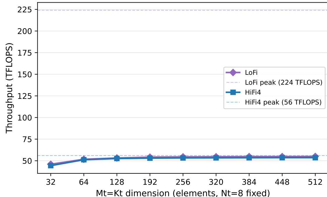
BF16: TFLOPS vs matrix size (INNER_LOOP=10000)
