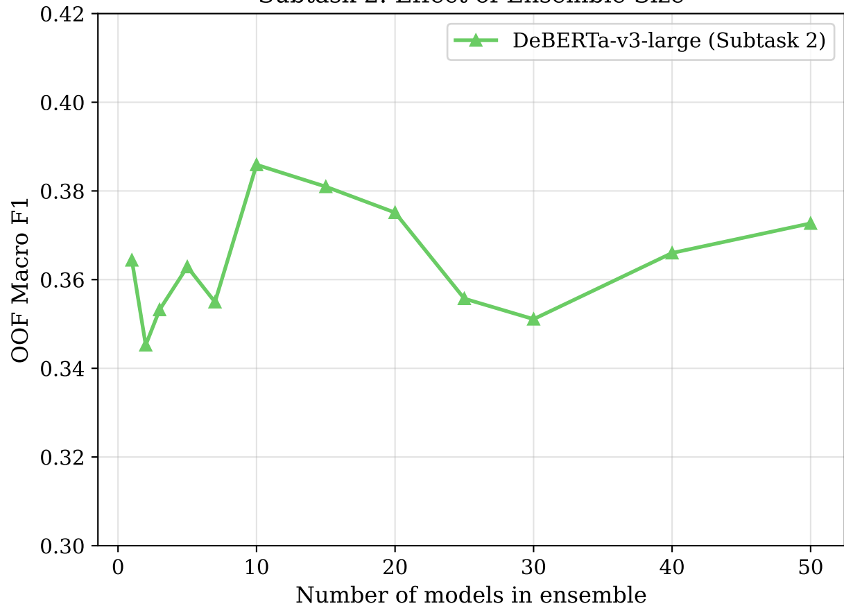
Subtask 2: Effect of Ensemble Size
