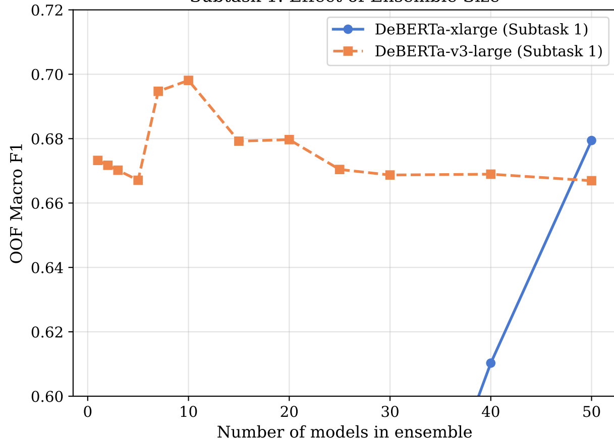
Subtask 1: Effect of Ensemble Size
