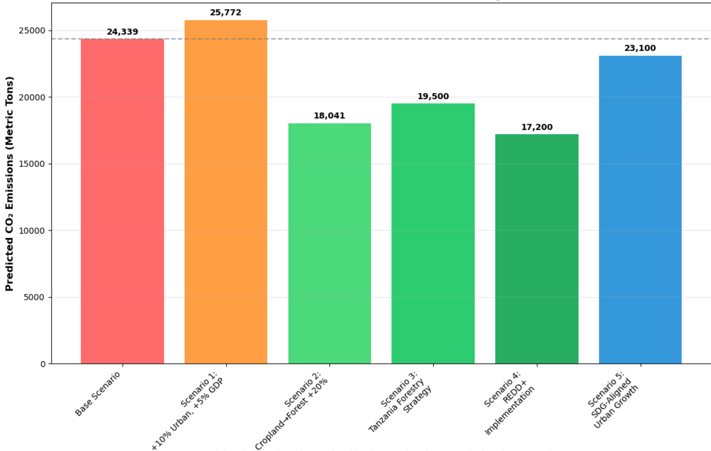
Predicted CO 2 Emissions Under Different Policy Scenarios
