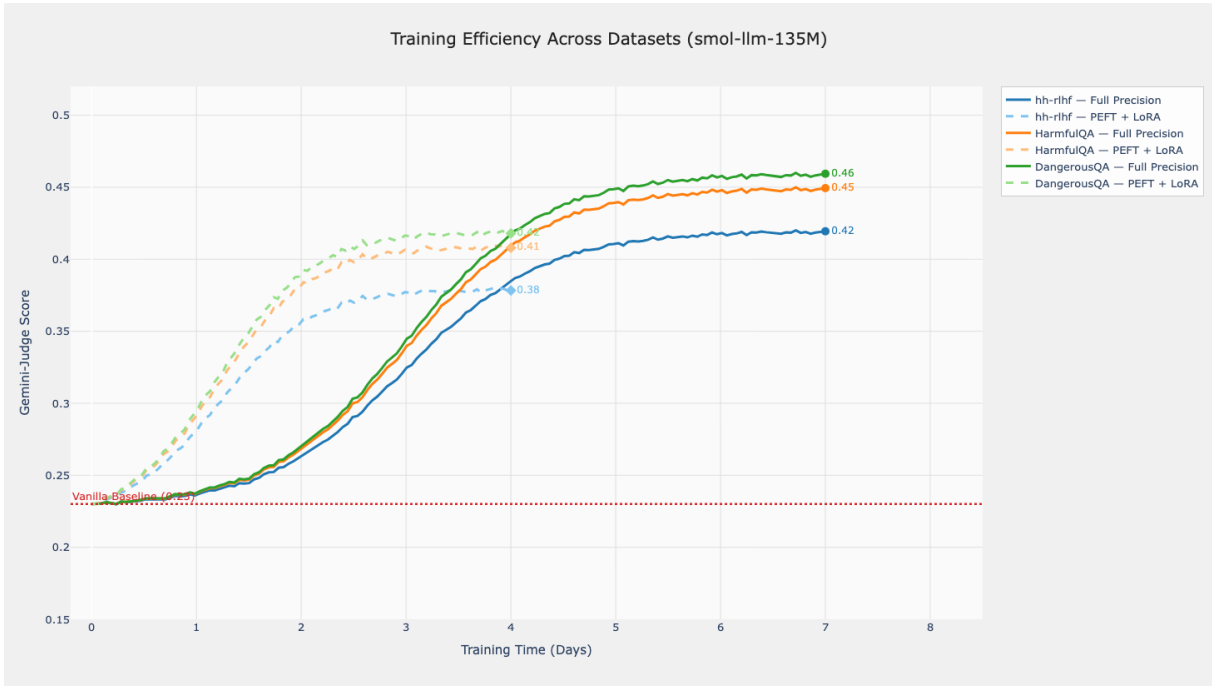
Figure 4: Training efficiency across datasets for SmolLM-135M. PEFT+LoRA reaches lower but comparable scores after roughly four days, while full fine-tuning continues to improve until roughly seven days.
