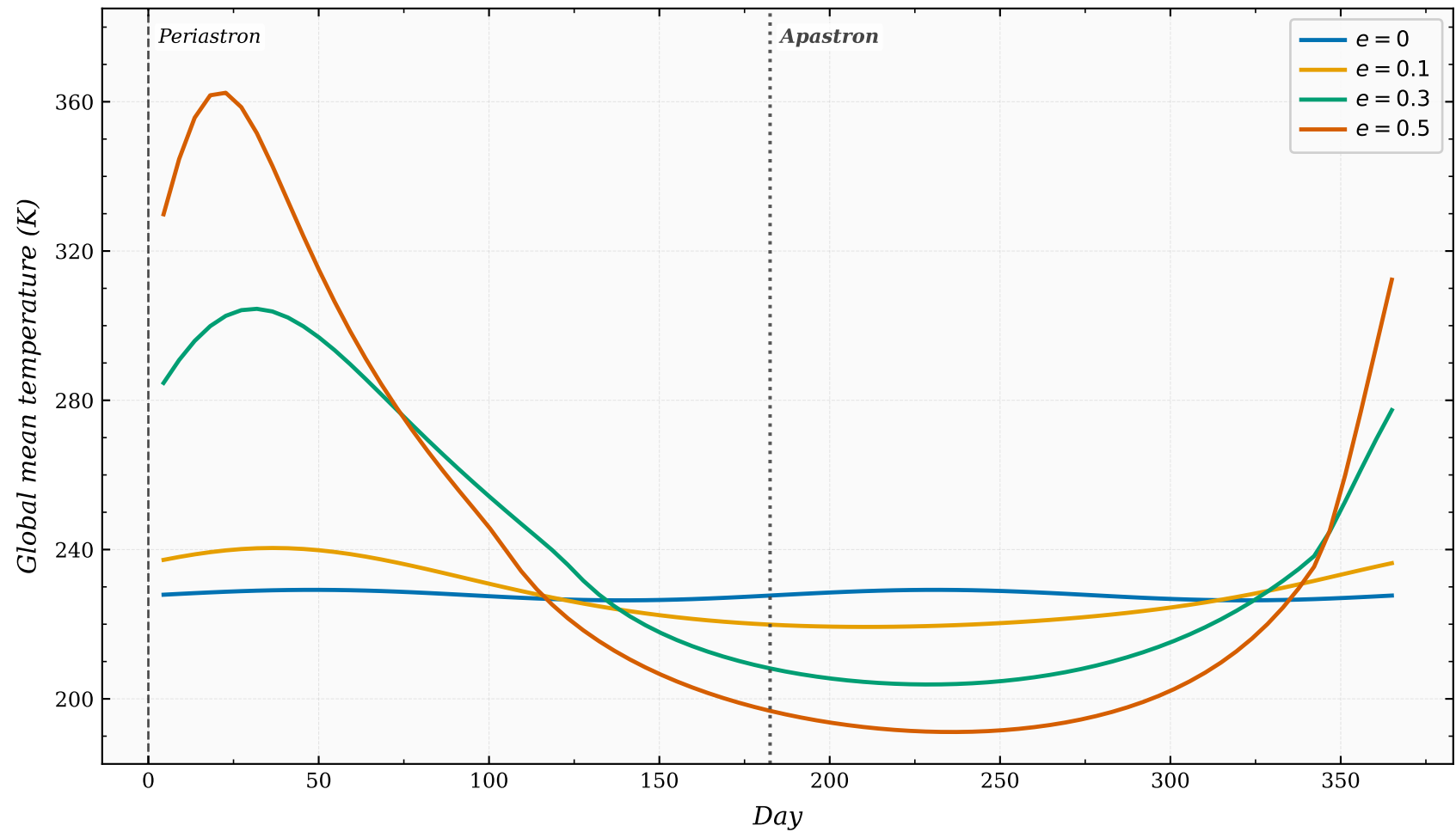
Seasonal temperature evolution for different eccentricities
