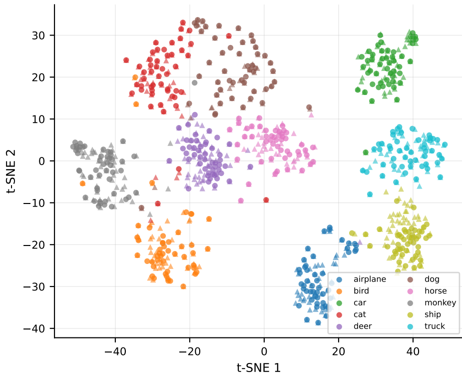
resnet50 — clean (o) vs hue90 (^) (perplexity=30, metric=cosine, seed=6304)
