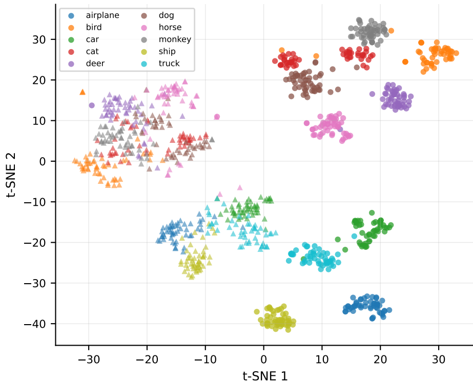
clip_vitb32 — clean (o) vs patch_shuffle (^) (perplexity=30, metric=cosine, seed=6304)
