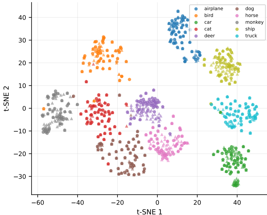
resnet50 — clean (o) vs grayscale (^) (perplexity=30, metric=cosine, seed=6304)
