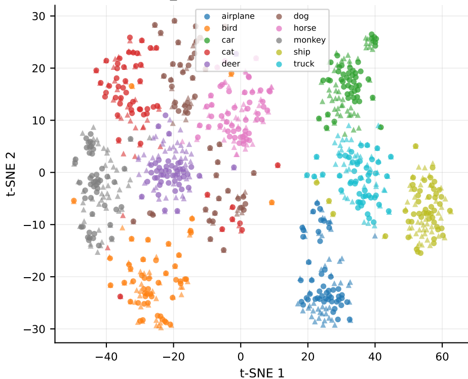
resnet50 — clean (o) vs patch_shuffle (^) (perplexity=30, metric=cosine, seed=6304)
