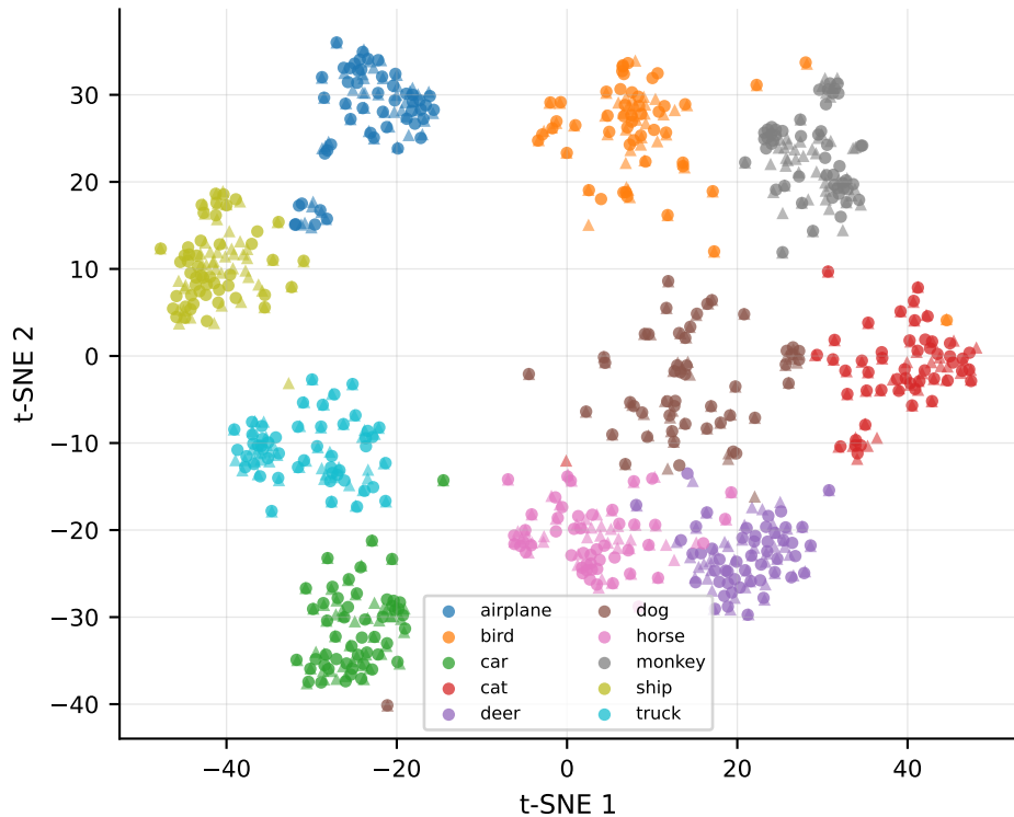
vit_b16 — clean (o) vs grayscale (^) (perplexity=30, metric=cosine, seed=6304)
